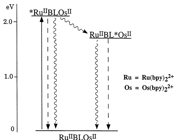
Fig. 5. Energy level diagram showing the photoinduced energy transfer deactivation process in \text{Ru}^{\text{II}}\text{-BL-Os}^{\text{II}} . Key: full line, excitation; dotted line, luminescence; wavy line, radiationless decay.
